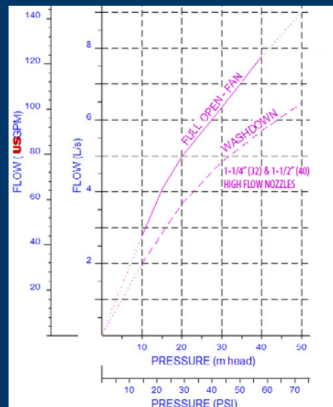
High Flow Nozzles 32 (1-1/4"), 40 (1-1/2")
