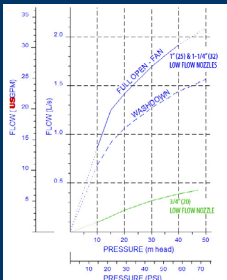
Low Flow Nozzles 20 (3/4"), 25 (1"), 32 (1-1/4")
